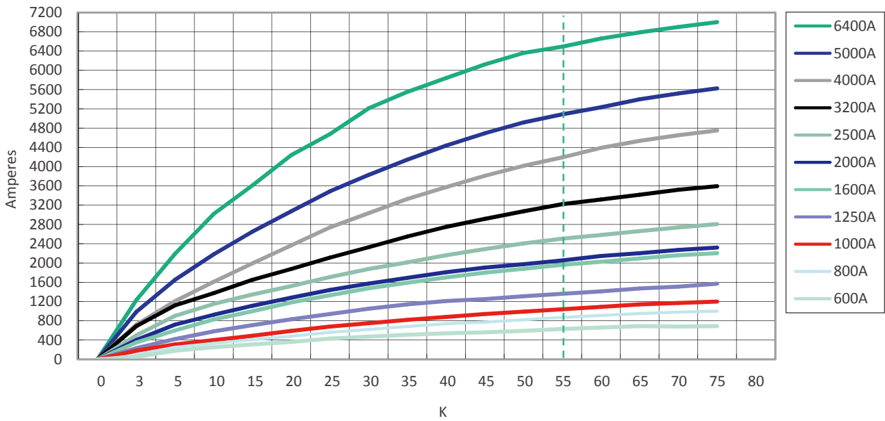
Temperature rise graph (Copper)
