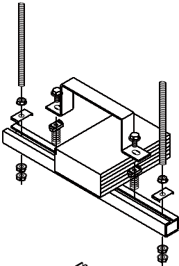
Ceiling trapeze
