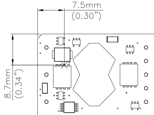
Figure 19: Temperature measurement location * The allowed maximum hot spot temperature is defined at 119°C.
