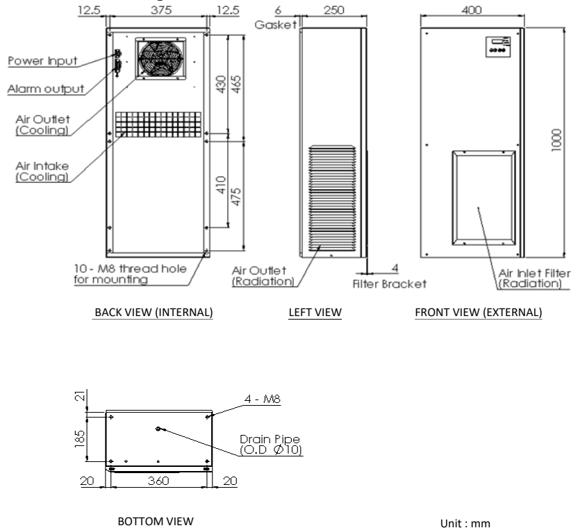
Dimension drawing
