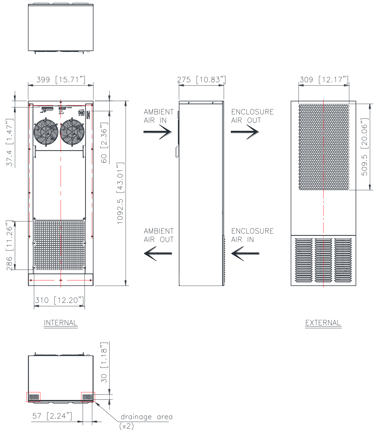
Dimension drawing
