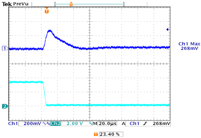
Figure 19: Typical transient response to step load change at 2.5A/\mu S from 100% to 50% of I_o , max at 5Vin, 3.3V out (Cout = ceramic, 10 \mu F tantalum)
