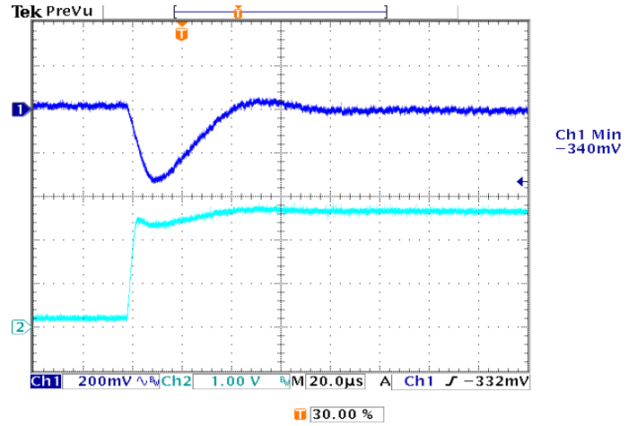
Figure 24: Typical transient response to step load change at 2.5A/\mu S from 50% to 100% of I_o , max at 3.3Vin, 2.5V out ( C_{out} = ceramic, 10\mu F tantalum)
