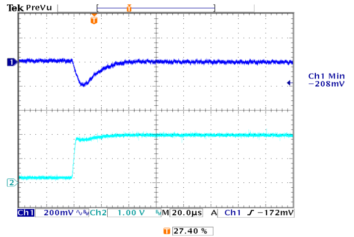
Figure 22: Typical transient response to step load change at 2.5A/\mu S from 50% to 100% of I_o , max at 5Vin, 1.8V out (Cout = ceramic, 10 \mu F tantalum)
