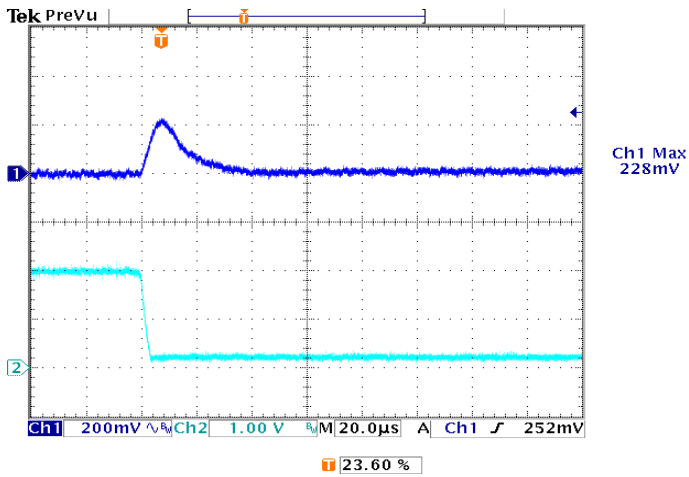
Figure 21: Typical transient response to step load change at 2.5A/\mu S from 100% to 50% of I_o , max at 5Vin, 1.8V out (Cout = ceramic, 10 \mu F tantalum)
