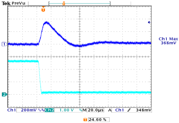
Figure 23: Typical transient response to step load change at 2.5A/\mu S from 100% to 50% of I_o , max at 3.3Vin, 2.5V out ( C_{out} = ceramic, 10\mu F tantalum)
