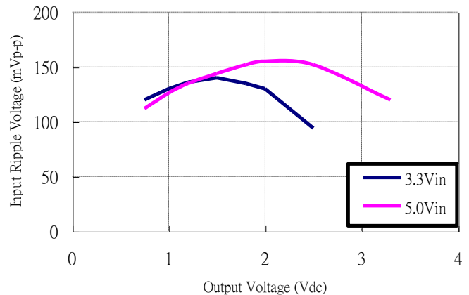
Figure 33: Input voltage ripple for various output models, I_O = 16 \text{ A} ( C_{IN} = 4 \times 100 \mu\text{F} tantalum // 2 \times 47 \mu\text{F} ceramic)
