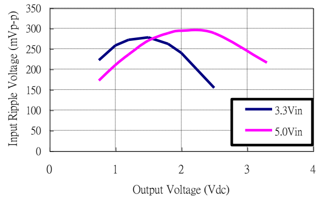
Figure 32: Input voltage ripple for various output models, I_O = 16 \text{ A} ( C_{IN} = 2 \times 100 \mu\text{F} tantalum // 47 \mu\text{F} ceramic)
