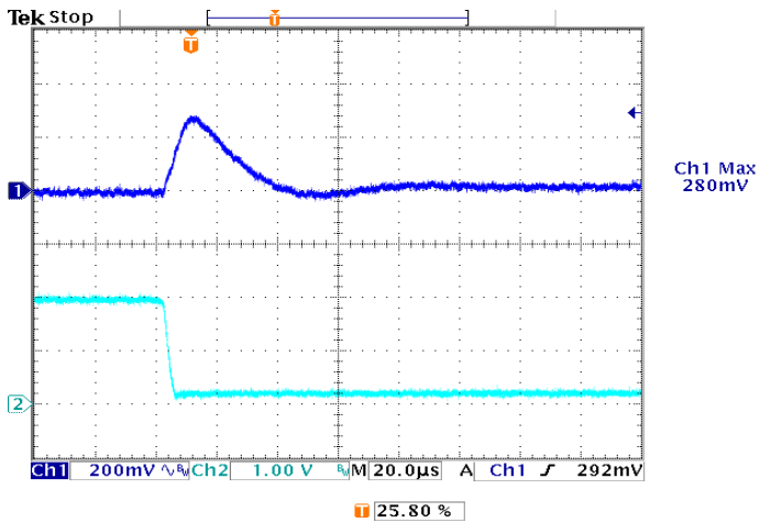
Figure 25: Typical transient response to step load change at 2.5A/\mu S from 100% to 50% of I_o , max at 3.3Vin, 1.8V out ( C_{out} = ceramic, 10\mu F tantalum)
