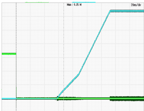
Figure 4: Remote On/Off(negative logic) at full load
