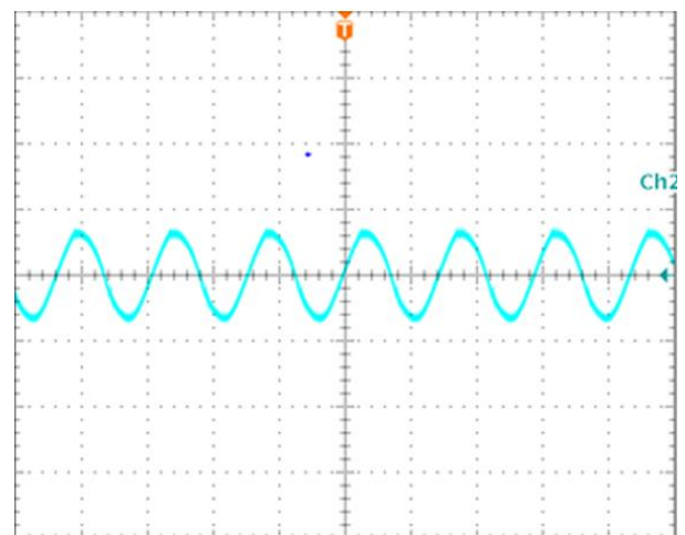
Figure 11: Output Voltage Ripple and Noise at nominal input voltage and max load current (50 mV/div, 2us/div) Load cap: 470μF Oscon cap. Bandwidth: 20MHz.
