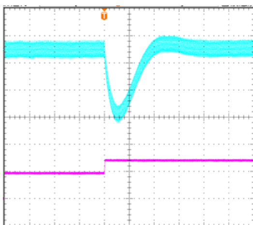
Figure 6: Transient Response
