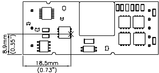
Figure 21: Hot spot temperature measured point. *The allowed maximum hot spot temperature is defined at 115°C
