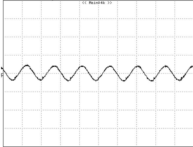
Figure 11: Input Terminal Ripple Current, i_c , at full rated output current and nominal input voltage with 12\mu\text{H} source impedance and 33\mu\text{F} electrolytic capacitor (100 mA/div, 2us/div).
