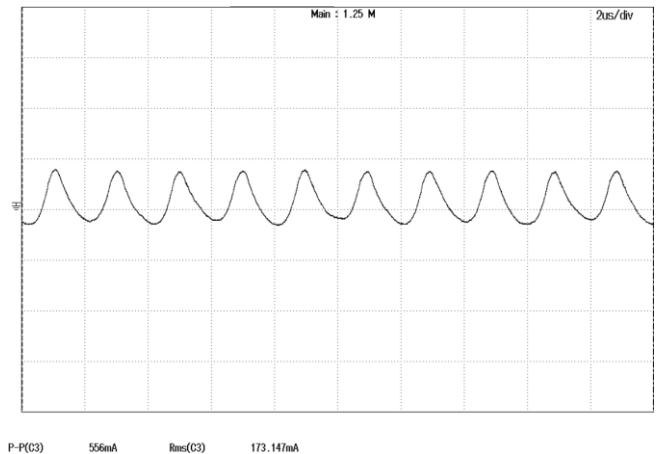
Figure 9: Input Terminal Ripple Current, i_c , at max output current and nominal input voltage with 12µH source impedance and 100µF electrolytic capacitor (500 mA/div, 2µs/div).
