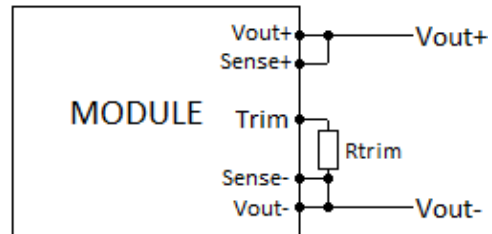
Figure 14: Circuit configuration for trim-down (decrease output voltage)
