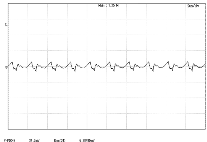
Figure 11: Output Voltage Ripple and Noise at nominal input voltage and max load current (50 mV/div, 2µs/div) Load cap: 470µF Oscon cap. Bandwidth: 20MHz.
