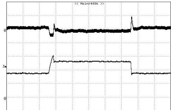
Figure 9: Output voltage response to step-change in load current (75%-50%-75% of I_o , max; di/dt = 1.0A/\mu s ). Load cap: 470 \mu F POS capacitor and 1 \mu F ceramic capacitor. Top Trace: V_{out} (100mV/div, 200 \mu s /div), Bottom Trace: I_{out} (10A/div). Scope measurement should be made using a BNC cable (length shorter than 20 inches). Position the load between 51 mm to 76 mm (2 inches to 3 inches) from the module
