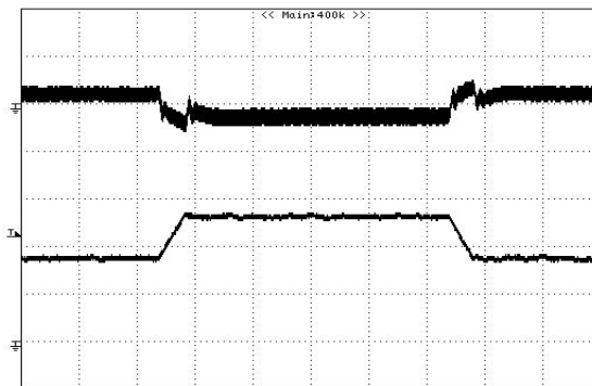
Figure 8: Output voltage response to step-change in load current (75%-50%-75% of I_o , max; di/dt = 0.1A/\mu s ). Load cap: 10 \mu F tantalum capacitor and 1 \mu F ceramic capacitor. Top Trace: V_{out} (50mV/div, 200 \mu s /div), Bottom Trace: I_{out} (10A/div). Scope measurement should be made using a BNC cable (length shorter than 20 inches). Position the load between 51 mm to 76 mm (2 inches to 3 inches) from the module
