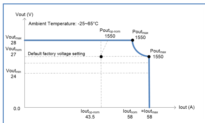
Output Characteristic
