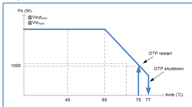
Temperature Characteristic
