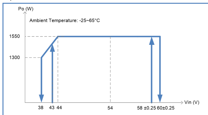
Input Characteristic
