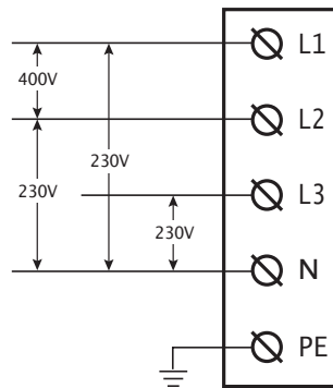
Figure 1. 380V - 415V Three-Phase Wiring Connection
