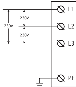
Figure 2. 200V - 230V Three-Phase Wiring Connection
