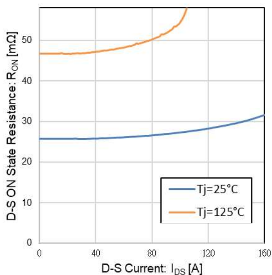
Fig 7. Typ. Drain-source on-state resistance
