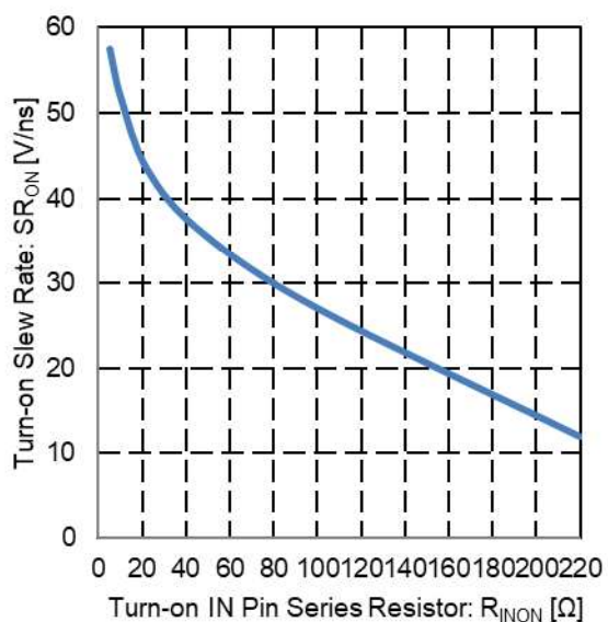
Fig 17. Turn-on Slew Rate vs Turn-on IN Pin Series Resistor
