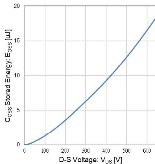
Fig 12. Typ. Coss stored energy
