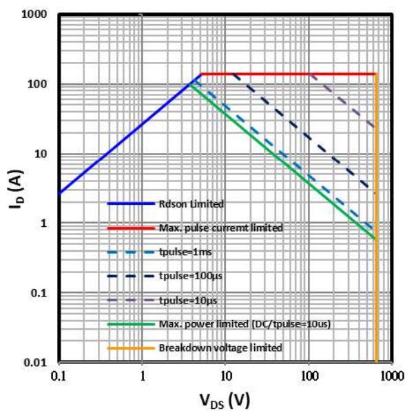
Fig 23. Safe operating area T_c=25^\circ C
