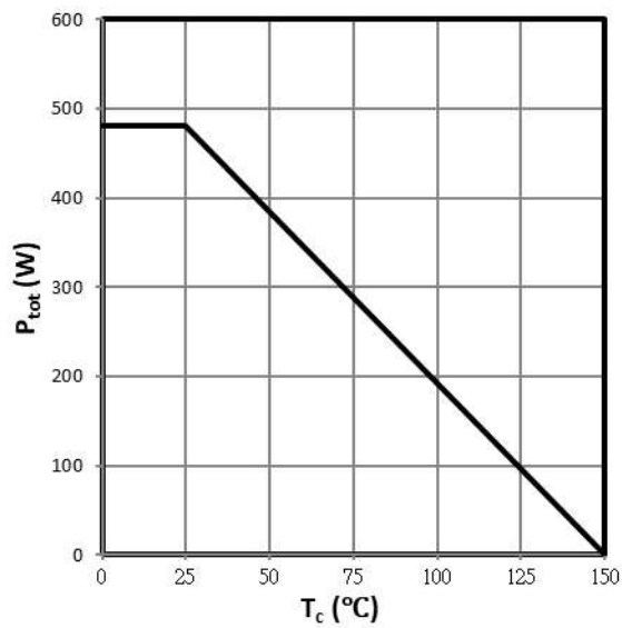
Fig 21. Power Dissipation
