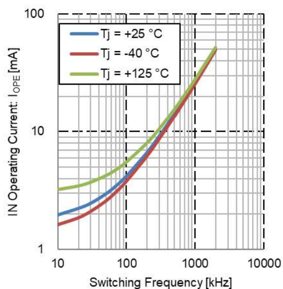
Fig 13. IN Operating Current vs Switching Frequency
