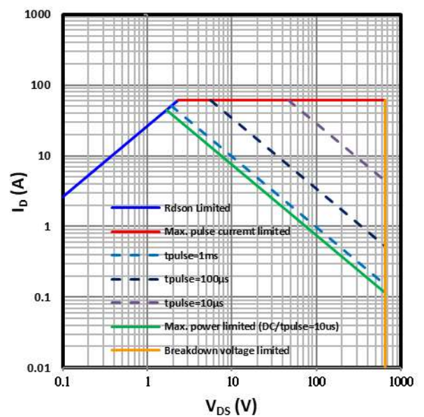
Fig 24. Safe operating area T_c=125^\circ C
