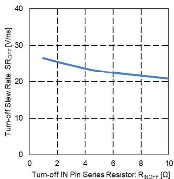
Fig 18. Turn-off Slew Rate vs Turn-off IN Pin Series Resistor
