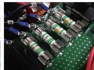
(String fuses)
