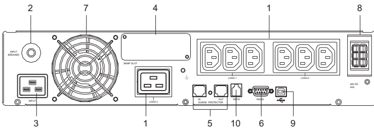
Figure 2-2.2 (2KVA & 3KVA Rear Panel)
