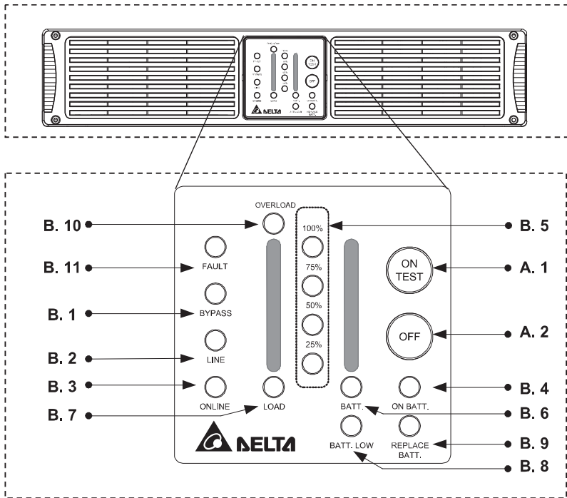
Figure 2-1 Operation Panel
