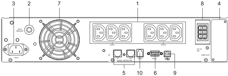
Figure 2-2.1 (1KVA Rear Panel)
