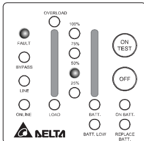
Figure 3-16 (Inverter O.V.P.)
