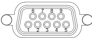
Figure 4-1 Pin Assignment
