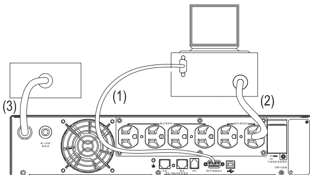
UPS Connector for 1KVA
