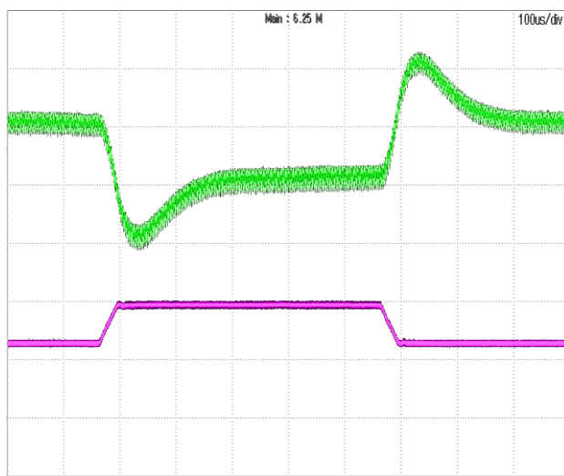
Top trace Vout dynamic AC value, 200mV/div, 100us/div Load cap: 33μF*5, Low ESR Polymer; 10μF Low ESR Polymer, 1μF ceramic capacitor Bandwidth: 20MHz
