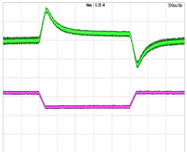
Top trace Vout dynamic AC Value, 200mV/div, 200us/div Load cap: 10μF Low ESR Polymer; 1μF ceramic capacitor 270μF*2 Low ESR Polymer; Bottom Trace :load 50% to 75% of rated Iout 10A/div, Bandwidth:20MHz
