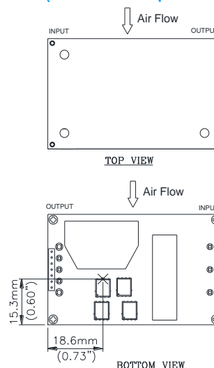
Figure 18: Hot spot 1 temperature measurement location
