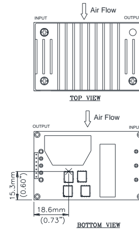
Figure 22: Hot spot 3 temperature measurement location
