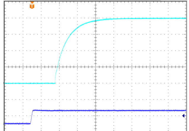
Turn-on transient at full load current (20ms/div). Top Trace: Vout; 3V/div; Bottom Trace: input voltage: 30V/div.
