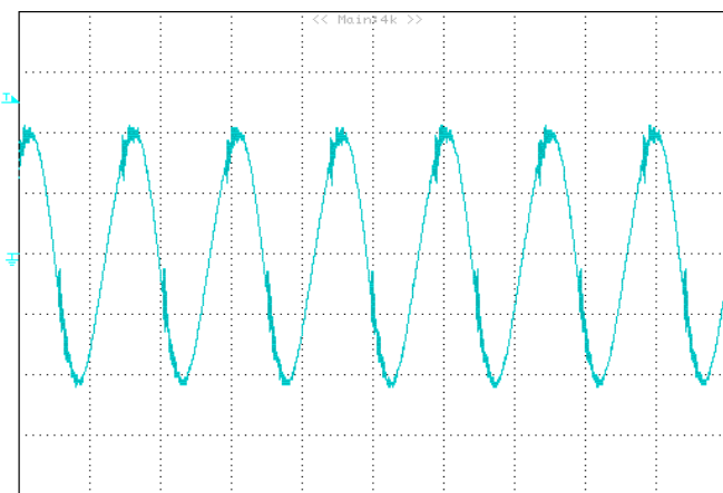
Output voltage ripple at nominal input voltage and max load current (20mV/div, 2us/div) Load cap: 10 \mu F, tantalum capacitor and 1 \mu F ceramic capacitor. Bandwidth: 20MHz.
