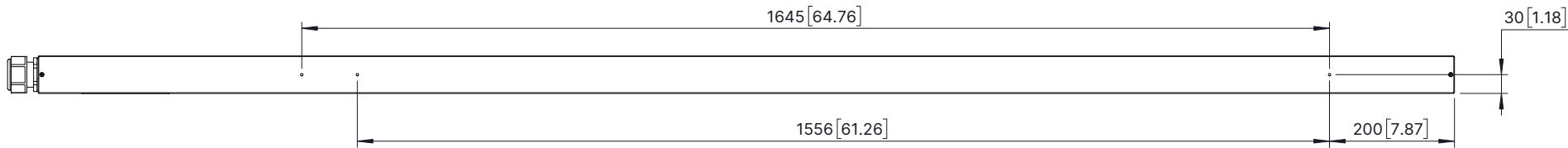
REAR VIEW
