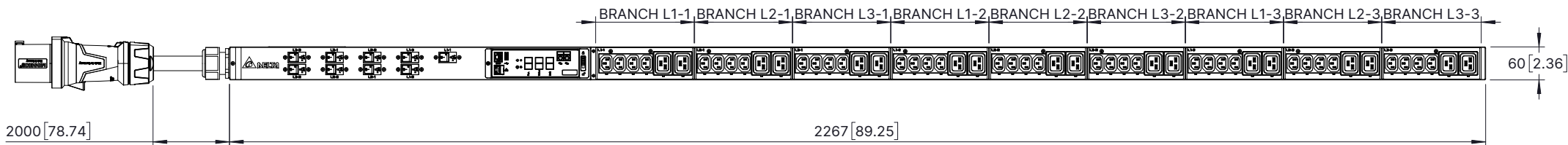
FRONT VIEW
